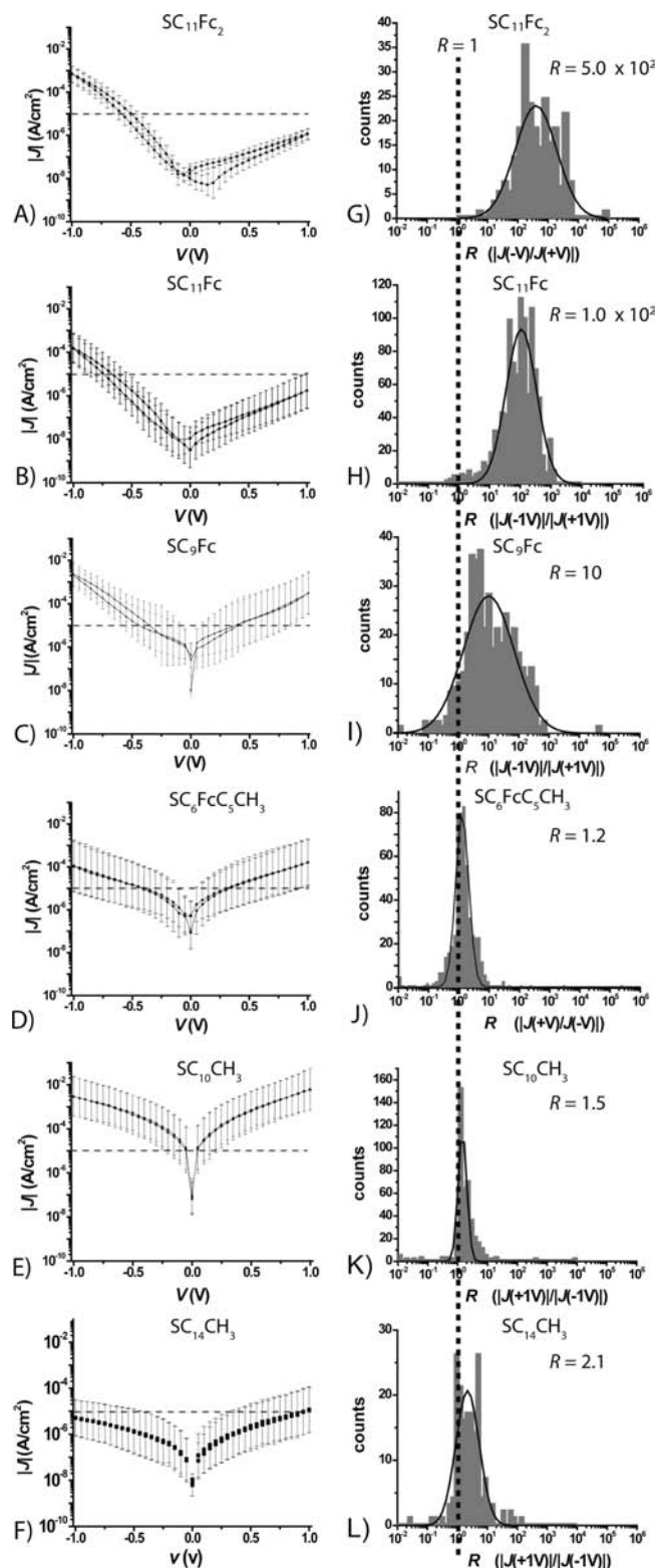
Figure 6. Average |J|(V) curves of the \text{Ag}^{\text{TS}}\text{-SC}_{11}\text{Fc}_2//\text{Ga}_2\text{O}_3/\text{EGaIn} (A), \text{Ag}^{\text{TS}}\text{-SC}_{11}\text{Fc}/\text{Ga}_2\text{O}_3/\text{EGaIn} (B), \text{Ag}^{\text{TS}}\text{-SC}_9\text{Fc}/\text{Ga}_2\text{O}_3/\text{EGaIn} (C), \text{Ag}^{\text{TS}}\text{-SC}_6\text{FcC}_5\text{CH}_3//\text{Ga}_2\text{O}_3/\text{EGaIn} (D), \text{Ag}^{\text{TS}}\text{-SC}_{10}\text{CH}_3//\text{Ga}_2\text{O}_3/\text{EGaIn} (E), and \text{Ag}^{\text{TS}}\text{-SC}_{14}\text{CH}_3//\text{Ga}_2\text{O}_3/\text{EGaIn} (F) junctions. The error bars are defined by the log-standard deviation, as in Figure 5 (see text). The dashed line is a guide for the eye placed at J = 10^{-5} \text{ A/cm}^2 . The histograms of the rectification ratios R = |J(+V)/J(-V)| at \pm 1 \text{ V} are shown with Gaussian fits to these histograms for the \text{Ag}^{\text{TS}}\text{-SC}_{11}\text{Fc}/\text{Ga}_2\text{O}_3/\text{EGaIn} (G), \text{Ag}^{\text{TS}}\text{-SC}_{11}\text{Fc}_2//\text{Ga}_2\text{O}_3/\text{EGaIn} (H), and \text{Ag}^{\text{TS}}\text{-SC}_9\text{Fc}/\text{Ga}_2\text{O}_3/\text{EGaIn} (I) junctions. The histograms of the rectification ratios R = |J(V)/J(-V)| at \pm 1 \text{ V} are shown with Gaussian fits to these histograms for the \text{Ag}^{\text{TS}}\text{-SC}_6\text{FcC}_5\text{CH}_3//\text{Ga}_2\text{O}_3/\text{EGaIn} (J), \text{Ag}^{\text{TS}}\text{-SC}_{10}\text{CH}_3//\text{Ga}_2\text{O}_3/\text{EGaIn} (K), and \text{Ag}^{\text{TS}}\text{-SC}_{14}\text{CH}_3//\text{Ga}_2\text{O}_3/\text{EGaIn} (L) junctions. The dashed line is a guide for the eye placed at R = 1 .
