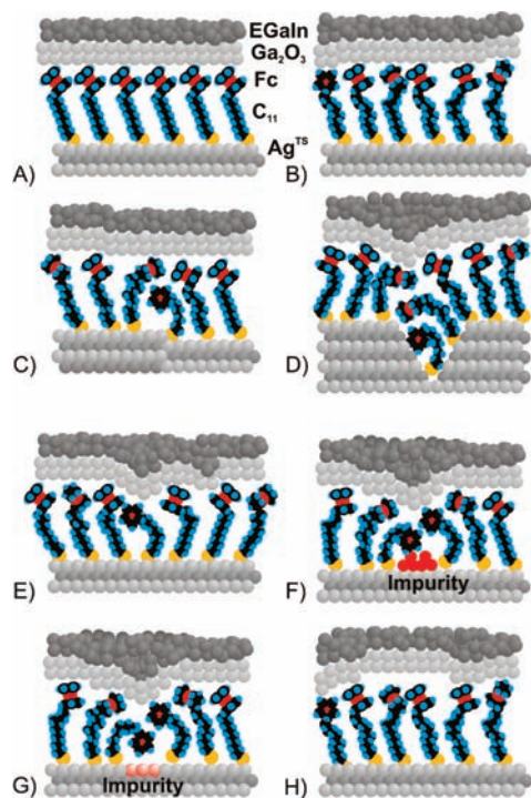
Figure 2. Schematic representations of several possible defects in \text{Ag}^{\text{TS}}\text{-SC}_{11}\text{Fc}/\text{Ga}_2\text{O}_3/\text{EGaIn} junctions: (A) a defect-free junction, and defects due to (B) Fc moieties having different orientations, (C) step-edges in the \text{Ag}^{\text{TS}} electrode (similar defects are also caused by vacancy islands), (D) grain boundaries of the \text{Ag}^{\text{TS}} electrode, (E) boundaries between domains in the SAM with different orientations of the alkyl chains, (F) physisorbed material, (G) impurities in the \text{Ag}^{\text{TS}} electrode (F and G may locally prevent adsorption of thiols), and (H) non-conformal contact of the \text{Ga}_2\text{O}_3/\text{EGaIn} top electrode with the SAM.
