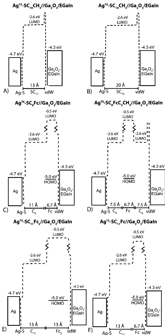
Figure 7. Energy level diagrams at open circuit for the \text{Ag}^{\text{TS}}\text{-SC}_{10}\text{CH}_3//\text{Ga}_2\text{O}_3/\text{EGaIn} (A), \text{Ag}^{\text{TS}}\text{-SC}_{14}\text{CH}_3//\text{Ga}_2\text{O}_3/\text{EGaIn} (B), \text{Ag}^{\text{TS}}\text{-SC}_9\text{Fc}/\text{Ga}_2\text{O}_3/\text{EGaIn} (C), \text{Ag}^{\text{TS}}\text{-SC}_6\text{FcC}_5\text{CH}_3//\text{Ga}_2\text{O}_3/\text{EGaIn} (D), \text{Ag}^{\text{TS}}\text{-SC}_{11}\text{Fc}_2//\text{Ga}_2\text{O}_3/\text{EGaIn} (E), and \text{Ag}^{\text{TS}}\text{-SC}_{11}\text{Fc}/\text{Ga}_2\text{O}_3/\text{EGaIn} (F) junctions. Dashed lines indicate the width and height of the barriers. The barrier presented by the alkyl chain has a barrier height, defined by the LUMO of the alkyl chain, of -2.6 \text{ eV} and a barrier width, defined by the length of the alkyl chain, of 1.3 \text{ nm} . The HOMO levels of the Fc and Fc 2 were estimated from the cyclic voltammograms (see text), and the LUMO level is approximately -0.4 \text{ eV} . 68,69 The width of the HOMO level of the Fc 2 is approximately twice that of the HOMO level of the Fc. The barrier width and height of the van der Waals interface (vdW) are not known and are discussed in more detail in the text. Ag-S represents the silver-thiolate bond; C 9 , C 11 , C 15 , and C 6 are alkyl chains; and Fc is ferrocene.
