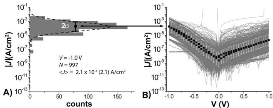
Figure 5. (A) Histogram of the values of J measured at V = −1.0 V obtained for Ag TS -SC 11 Fc//Ga 2 O 3 /EGaIn junctions, with a Gaussian fit to this histogram giving the log-mean value of J ( \mu_{\log} ) and the log-standard deviation ( \sigma_{\log} ). The values of \mu_{\log} at each V are plotted in the average trace (B, black squares), where the error bars (white) are located a factor of \sigma_{\log} above and below the log-mean, respectively. (B) Average trace of the Ag TS -SC 11 Fc//Ga 2 O 3 /EGaIn junctions superimposed over all 997 traces (gray) collected on these junctions. The three traces from junctions that short-circuited lie outside the scale of the figure ( |J| \approx 10^4 ) and are not shown.
