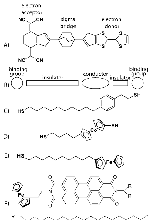
Figure 3. Several proposed molecular diodes. Aviram and Ratner proposed molecular diodes that contain electron donor and acceptor groups (A). Another class of proposed molecular diodes has a single molecular level (HOMO or LUMO), asymmetrically separated from the electrodes by two insulating groups of different lengths (B). Williams et al. 1 proposed a molecular rectifier with an asymmetrically coupled LUMO level (C), while Baranger et al. 2 proposed a rectifier with an asymmetrically coupled HOMO level (D). The latter is similar to the molecular rectifier that is used in the present study (E). Metzger et al. experimentally investigated a proposed molecular diode (F) consisting of a donor (Fc)–alkyl bridge ( \sigma )–acceptor (perylene) and functionalized with long alkyl chains ( C_{19} ).
