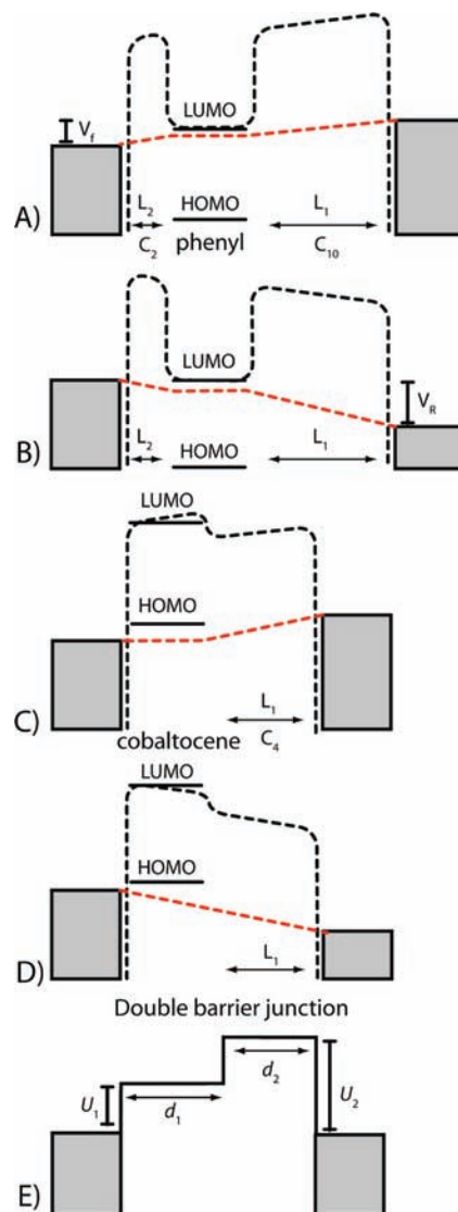
Figure 4. Mechanisms of rectification proposed by Williams 1 (A,B) and Baranger et al. 2 (C,D). The junction consists of two electrodes that contact the molecular diode (i.e., SC_{10} -phenyl- C_2S (Figure 3B) or SC_4CoS (Co = cobaltocene, Figure 3C)), with its LUMO or HOMO level energetically located just above the Fermi levels of the electrodes. The Fermi levels of the electrodes are equal. The width of the junction is determined by the length of the molecule. The spatial position of the LUMO is determined by the relative lengths of the alkyl spacers, i.e., L_1 and L_2 (for SC_{10} -phenyl- C_2S , L_1 = C_{10} and L_2 = C_2 ; for SC_4CoS , L_1 = C_4 and L_2 = 0 ). (A,C) Operation at forward bias: the current rises when the Fermi levels align with the conducting molecular level (at V = V_f ). (B,D) Operation at reverse bias, showing that greater bias is necessary than at forward bias in order to align the Fermi levels with the conducting molecular orbital. Ford et al. 35 analyzed a general two-barrier system to calculate the values for R as a function of barrier widths ( d_1 and d_2 ) and heights ( U_1 and U_2 ). Panel E shows this barrier for d_2/d_1 = 1 and U_2/U_1 = 0.5 .
